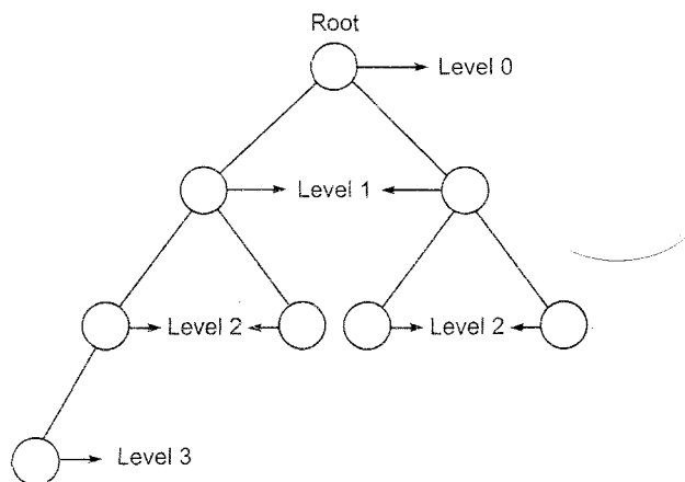
Fig. 2.10 Illustration of levels of vertices.
