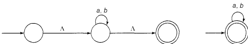
Fig. 5.25 Transition system for (a + b)^* .
