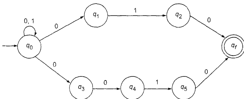
Fig. A5.4 NDFA for Exercise 5.12.
