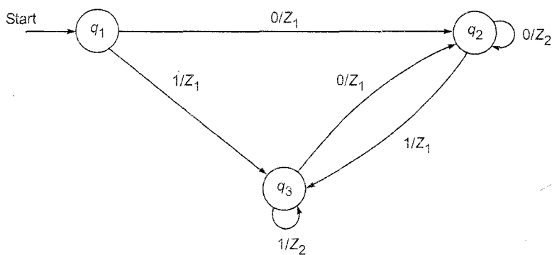
Fig. 3.10 Mealy machine of Example 3.12.
