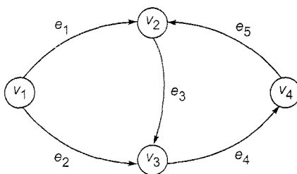
Fig. 2.4 A directed graph.
