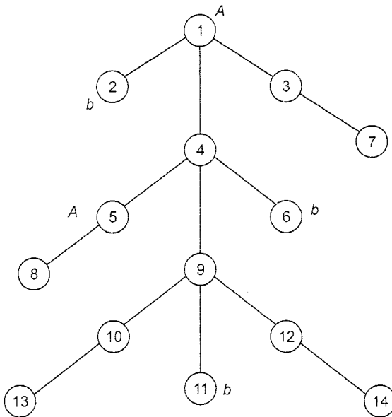
Fig. 6.14 Derivation tree for Question 1(e).
